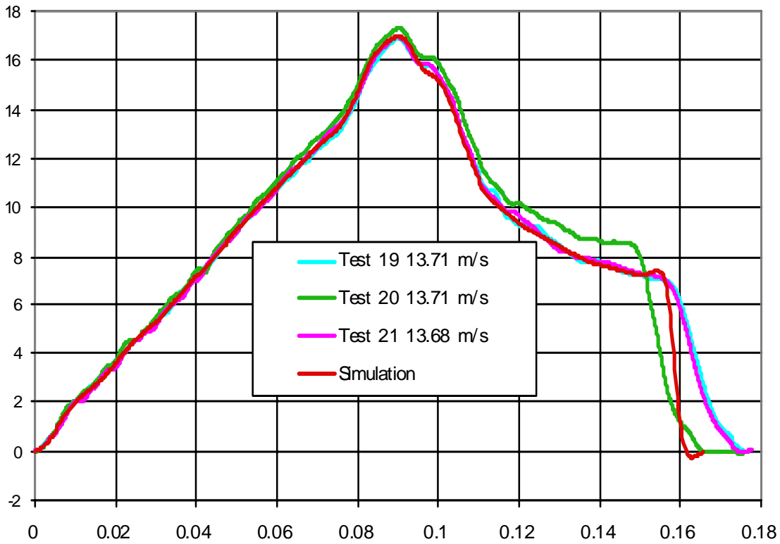
FAR 25.562 - 14g Down Test
