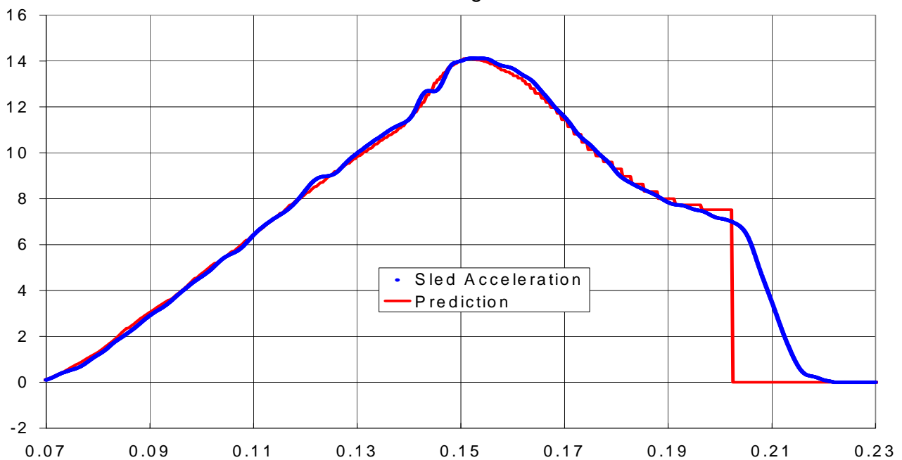
FAR 25.562 - 14g Down Test
