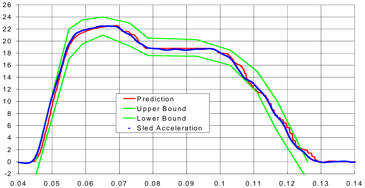
FMVSS 213 - Decelerator Sled
