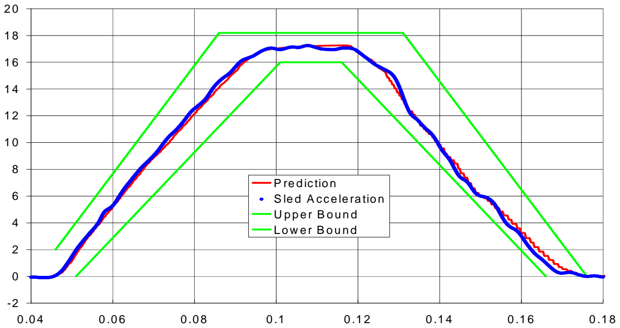
FMVSS208 - Decelerator Sled
